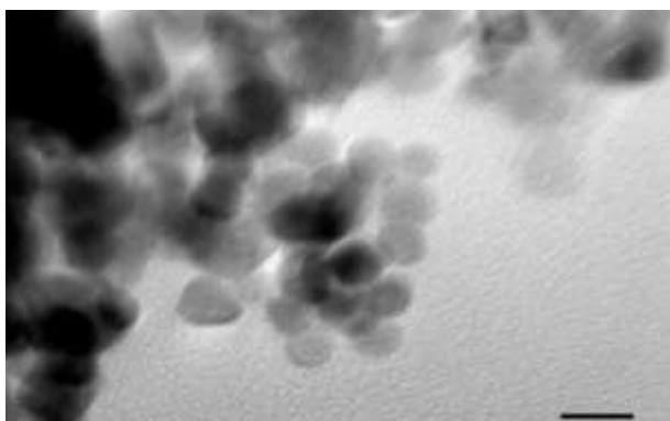
Figure 5 : HRTEM images of Mg 10% doped \text{Al}_2\text{O}_3 calcined at 600^\circ\text{C} for 2hrs
