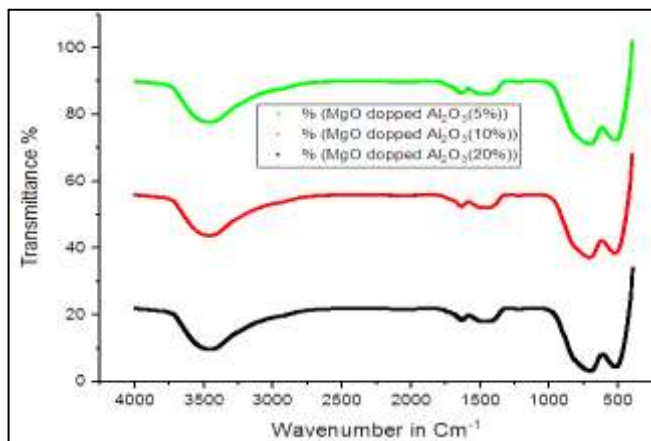
Figure 4: The IR spectra of samples calcined at 600^\circ\text{C} for 2 hours (a) MgO doped \text{Al}_2\text{O}_3 (5%) (b) MgO doped \text{Al}_2\text{O}_3 (10%) (c) MgO doped \text{Al}_2\text{O}_3 (20%)
